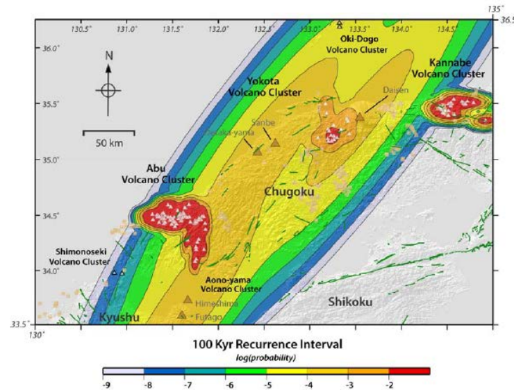
Figure 5.12: Probability of a new volcano or volcanic system forming within a 25 \text{ km}^2 area during the next 100 kyr contoured as the logarithm of probability to illustrate order of magnitude changes across the Chugoku region. Symbols as in Figure 5.1.
